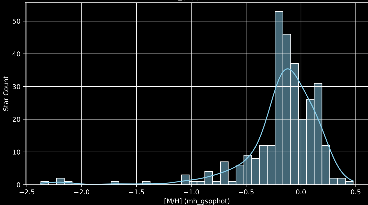
APOGEE DR17 Field: [191-08 [M/H] (mh_gspphot) (n= 301)
