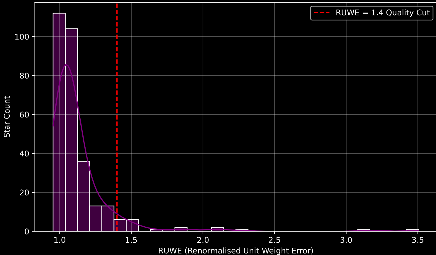
GAPOGEE DR17 Field [191-08] RUWE Distribution (n= 299)
