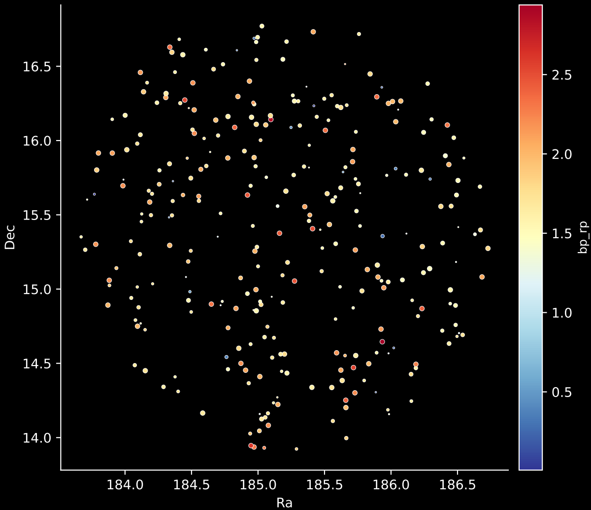
APOGEE DR17 Field: [191-08] Stars: 304
