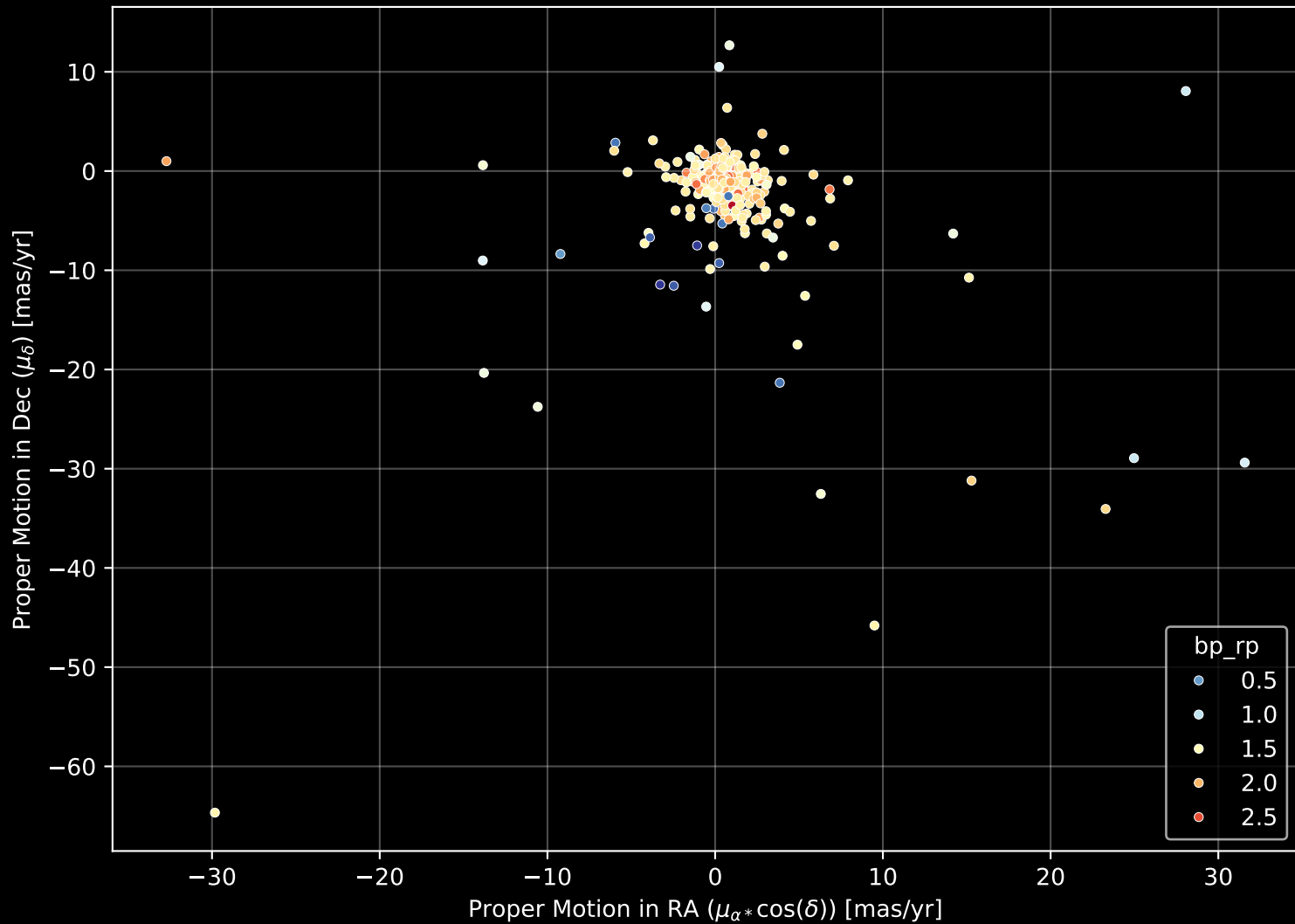
APOGEE DR17 Field: [191-08] Proper Motion Diagram (n= 304)
