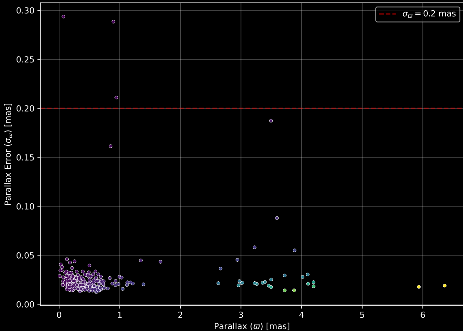
APOGEE DR17 Field: [191-08] Parallax Quality (n= 304)
